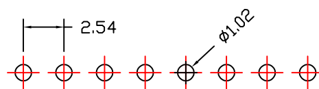
PCB LAYOUT
